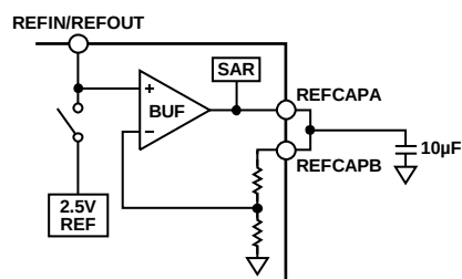
Figure 34. Reference Circuitry
