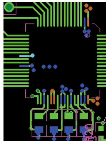
Figure 41. Top Layer Decoupling REFIN/REFOUT, REFCAPA, REFCAPB, and REGCAP Pins
