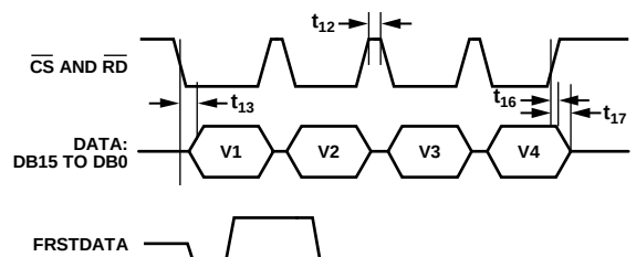
Figure 5. \overline{CS} and \overline{RD} , Linked Parallel Mode
